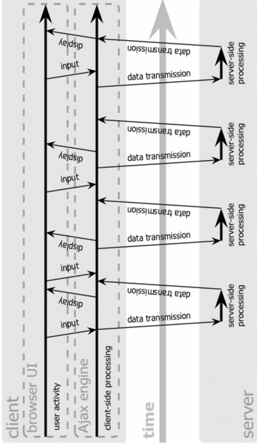
Ajax web application model (asynchronous)
