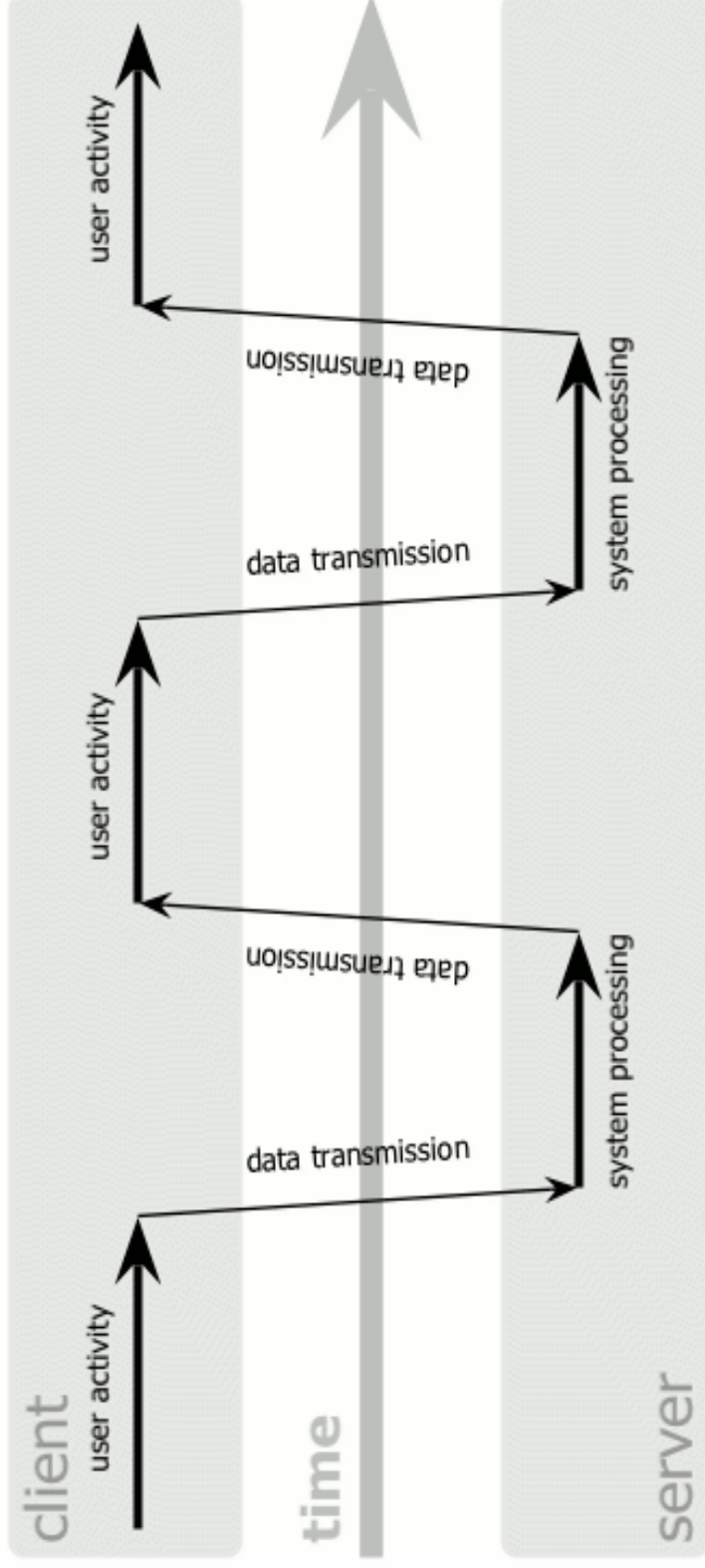
classic web application model (synchronous)
